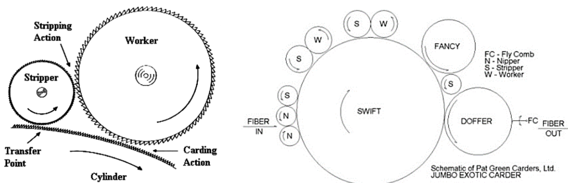
Figure. 4. Illustrates machines architecture of carding unite machine for recycling of low grade clothing Waste.
